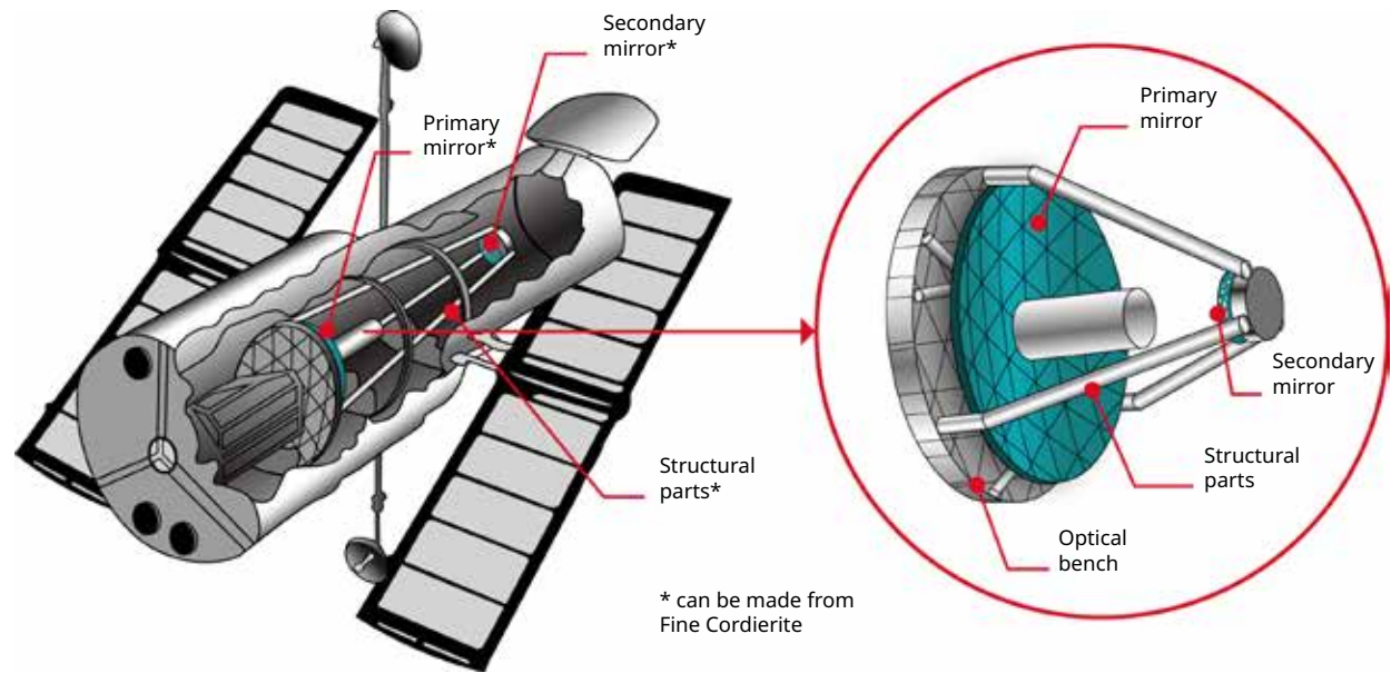
Structural parts made of ceramics in a satellite
