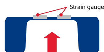
Piezo-resistive pressure measurement
