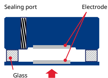
Capacitive pressure measurement
